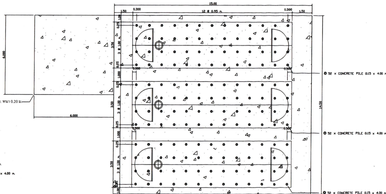
PLAN OF FOUNDATION
