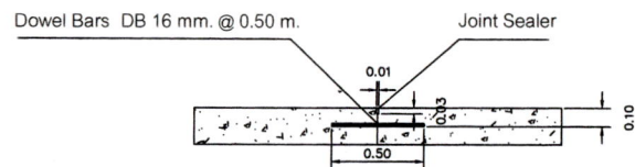
Construction Joint
