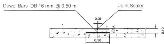
Construction Joint
