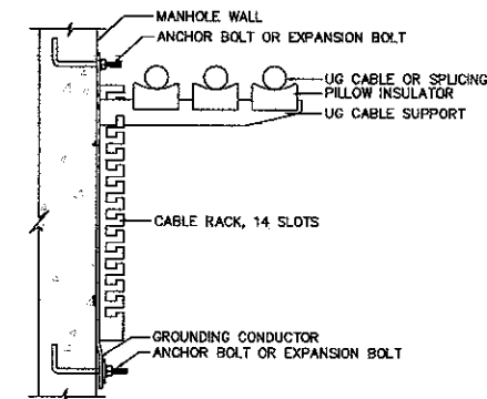
TYPICAL INSTALLATION OF UG CABLE RACK SUPPORT AND PILLOW INSULATOR FOR SUPPORTING UG CABLE AND SPLICING
