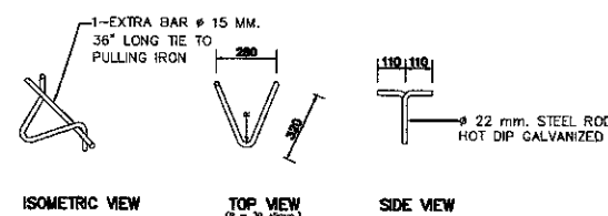
PULLING IRON DETAIL
