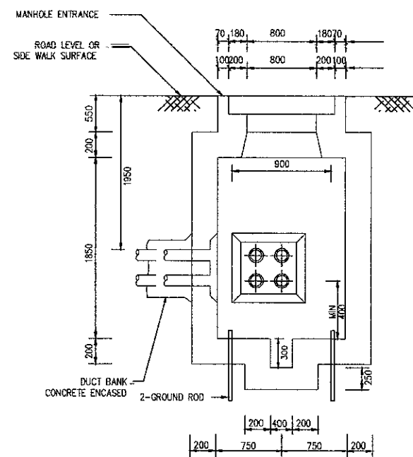
SECTION B-B
