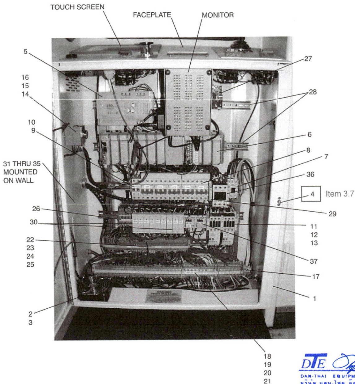
LOWER CONTROL CONSOLE
