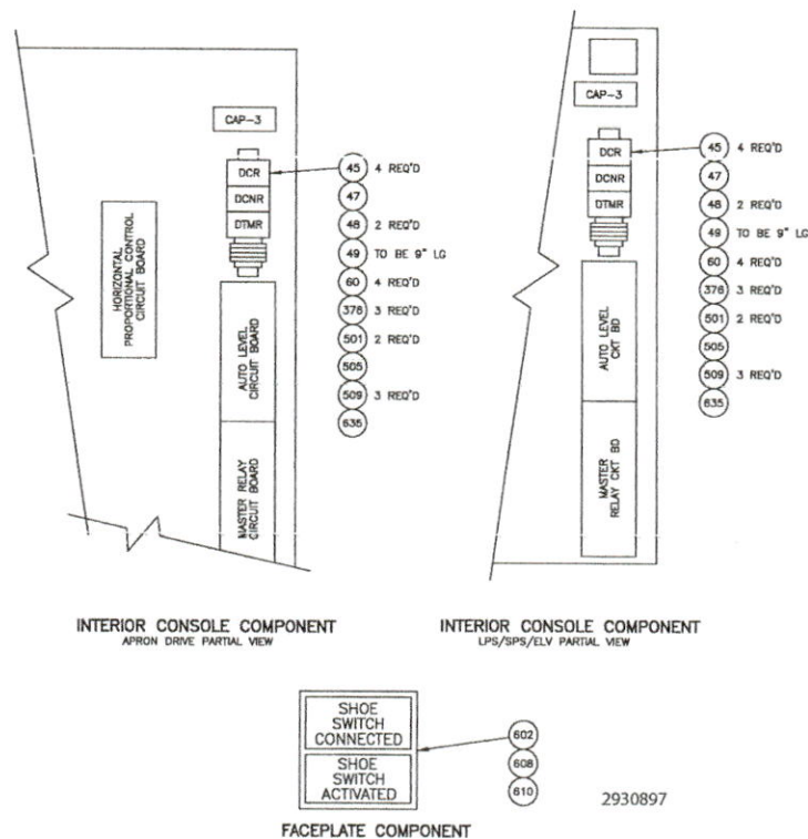
Figure 4. Solid-state autolevel safety switch installation
