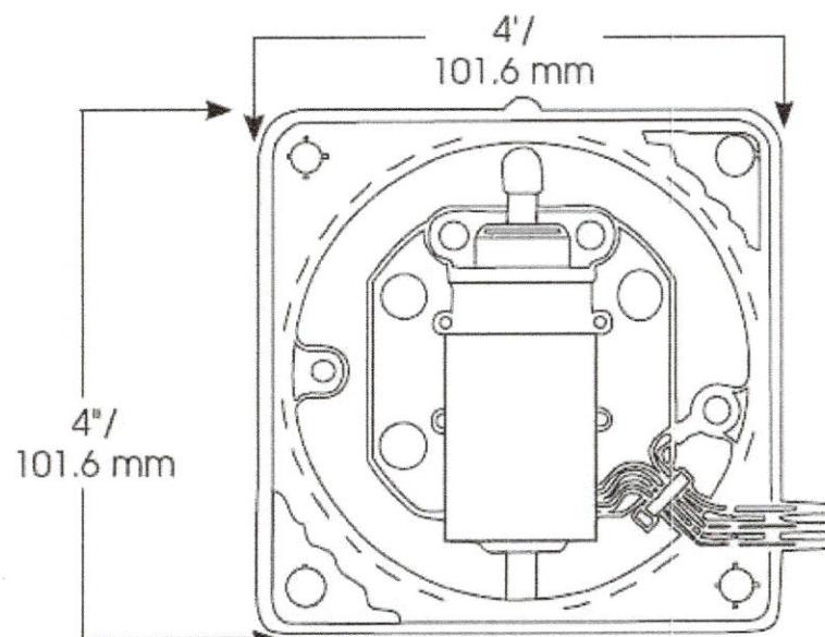
Back View Mechanisms
