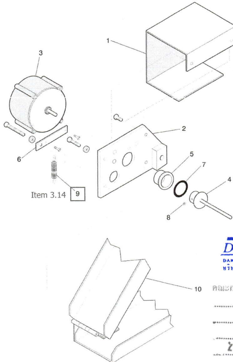
Cable Lifting Arm / Height Indicator Assembly
