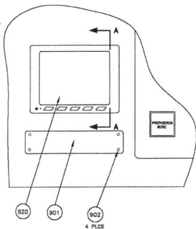
OLD CRT MONITOR CUTOUT (5.25"X4")
