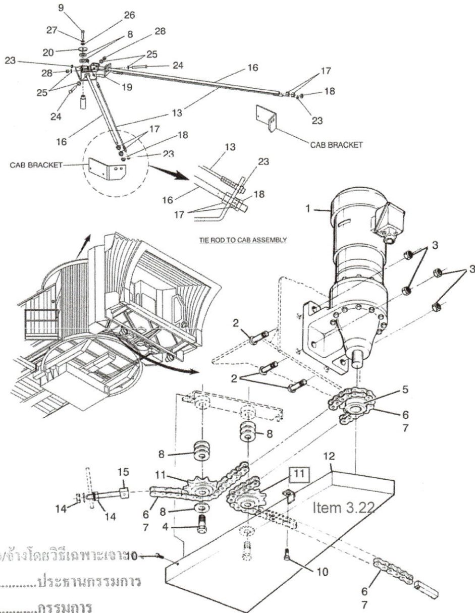
Cab Rotation Assembly
