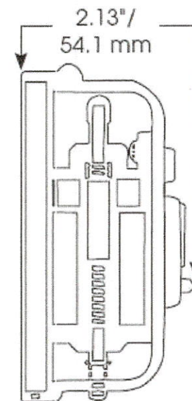
Side View Mechanisms
