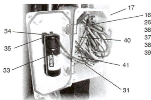
DETAIL A AUTOLEVEL JUNCTION BOX
