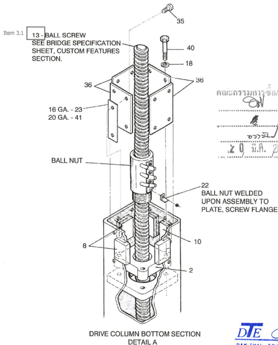
Vertical Lift Column
