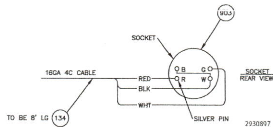
Figure 2. Cable and socket assembly wiring
