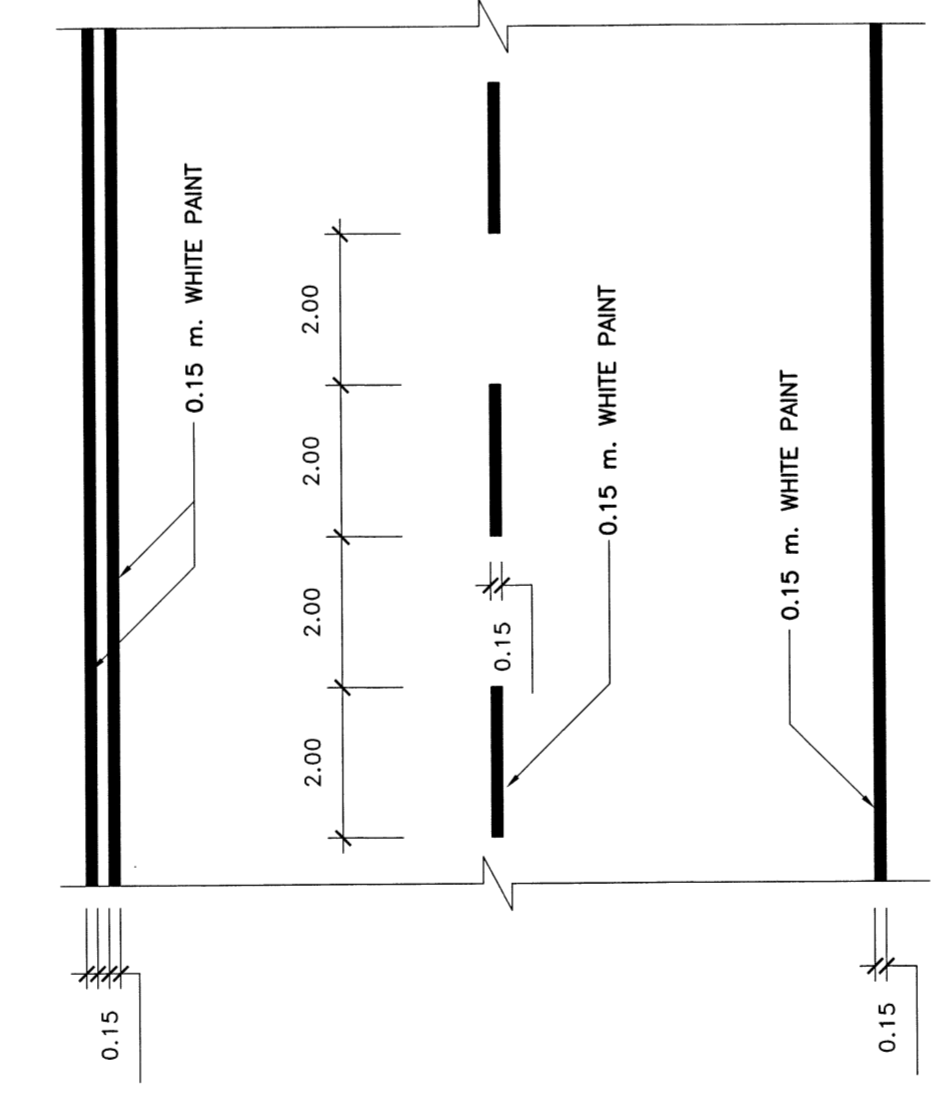
SERVICE ROAD MARKING NOT TO SCALE
